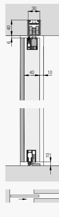
Hawa Porta 100 HMT Pocket Acoustics
