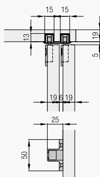
Hawa Clipo 16 H IS
