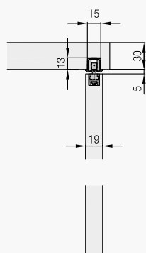
Hawa Clipo 16 HM IS
