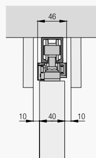
Hawa Junior 80 Z Symmetric
