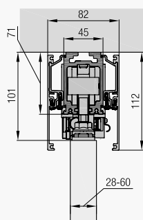
Hawa Frontslide 140 matic
