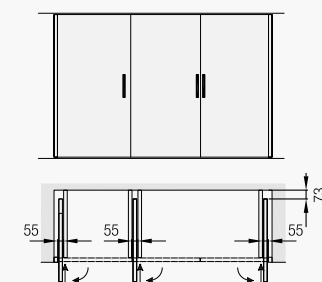
Hawa Concepta 25/30 Hawa Concepta 40/50
