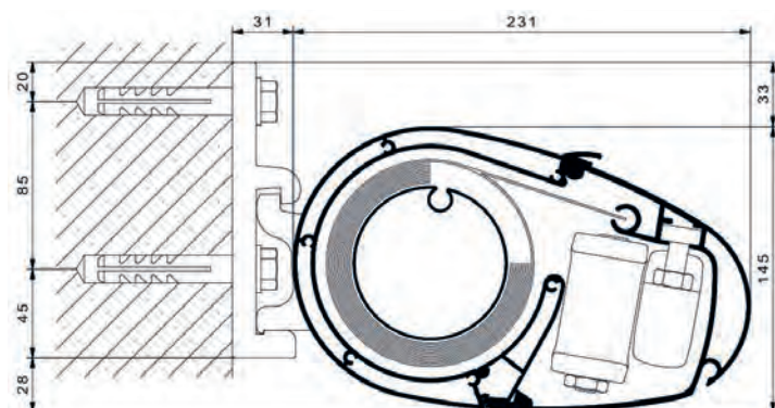
Wandmontage
