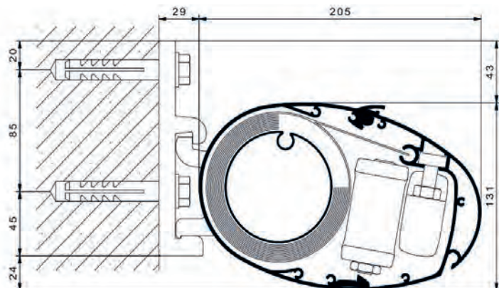
Wandmontage
