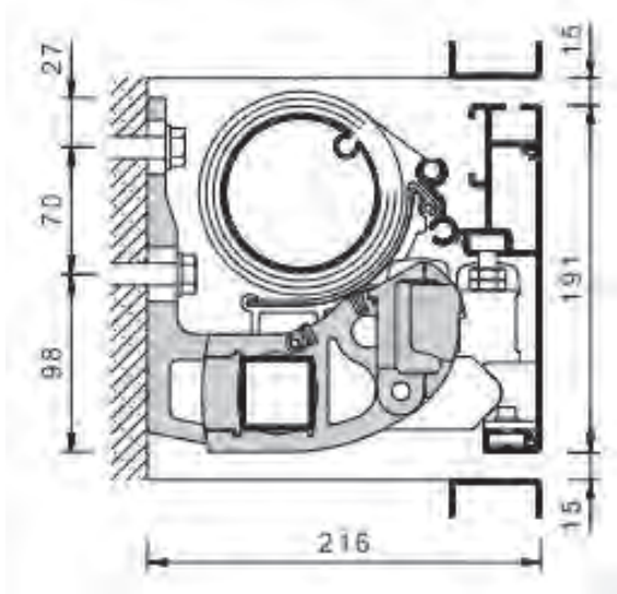
Wandmontage
