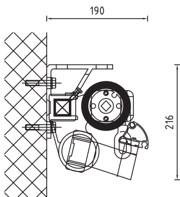
WANDMONTAGE
