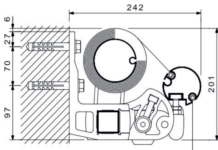
Wandmontage
