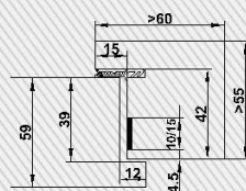
CombiModul-Blockrahmen
