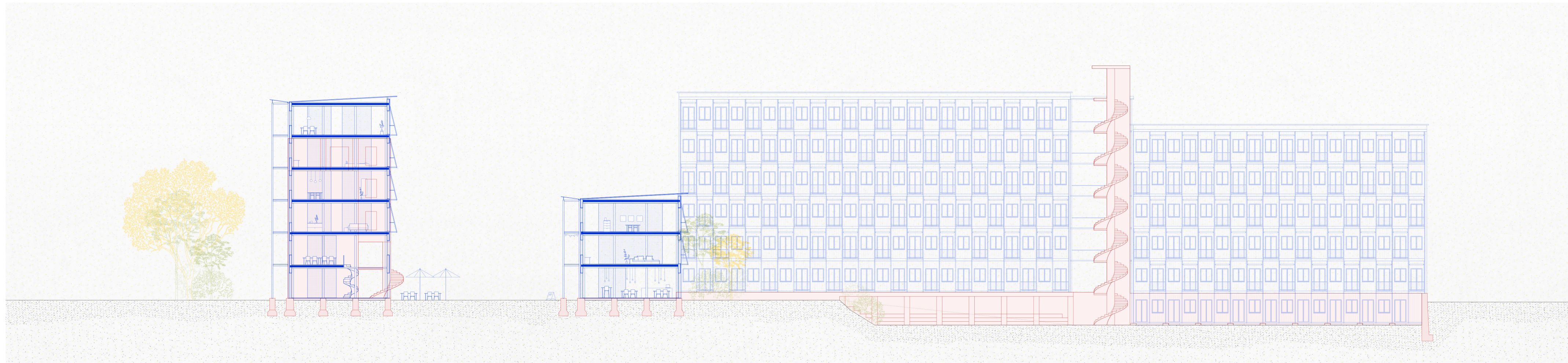
FROM MONOCULTURE TO A BUILDING ROTATION SYSTEM section east-west - overlay construction
