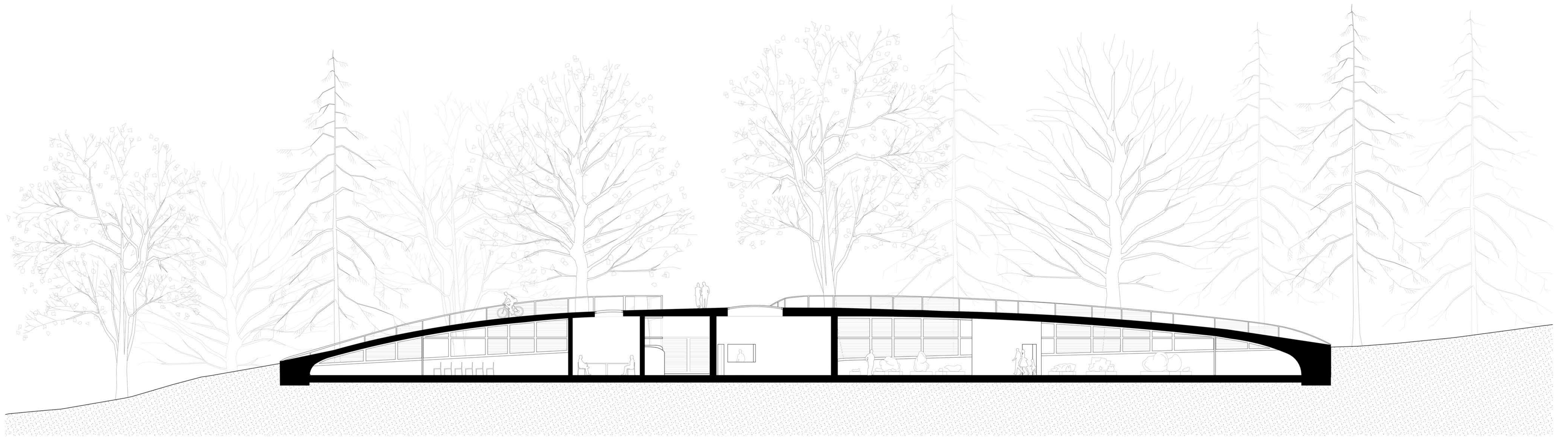
SECTION 1-1, 1:100
