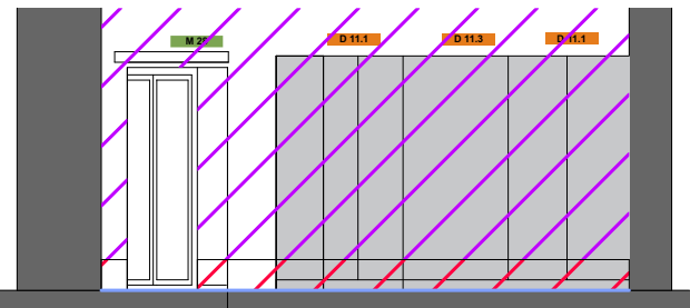
ELEVATION D-D 1: 75
