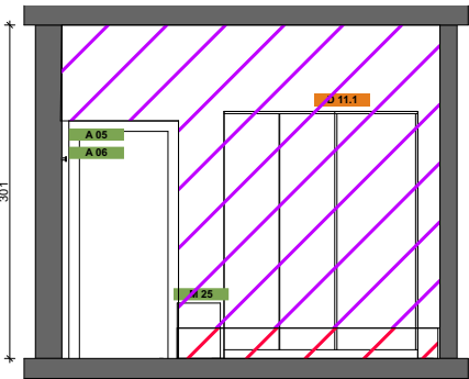
ELEVATION D-D 1: 75
