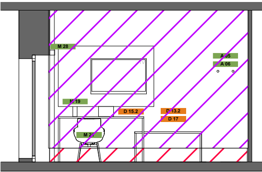
ELEVATION B-B 1: 75
