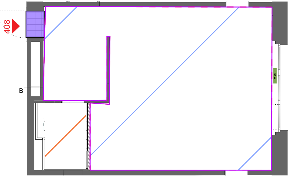
PLAN REVETMENTS MUR/ SOL 1: 100
