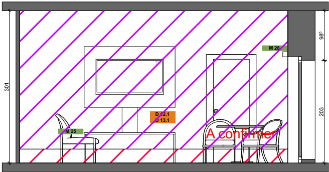
ELEVATION A-A 1: 75
