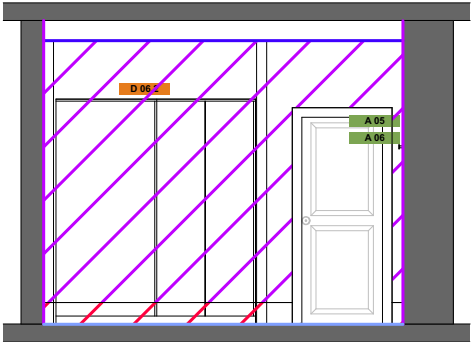
ELEVATION A-A 1: 75
