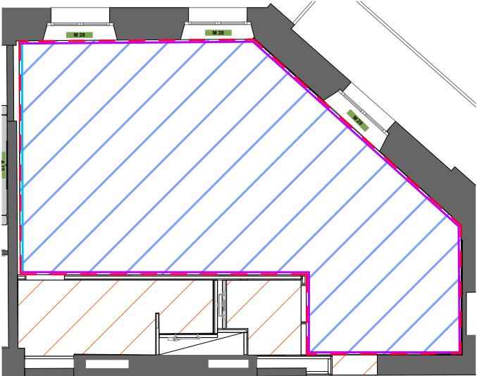
PLAN REVETMENTS MUR/ SOL 1: 75
