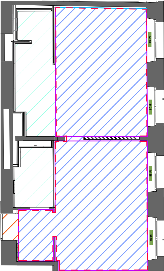
PLAN REVETMENTS MUR/ SOL 1: 75
