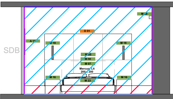
ELEVATION C-C 1: 75
