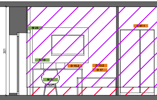
ELEVATION B-B 1: 75
