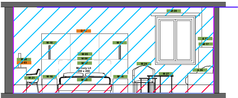
ELEVATION A-A 1: 75
