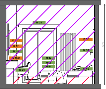
ELEVATION C-C 1: 75
