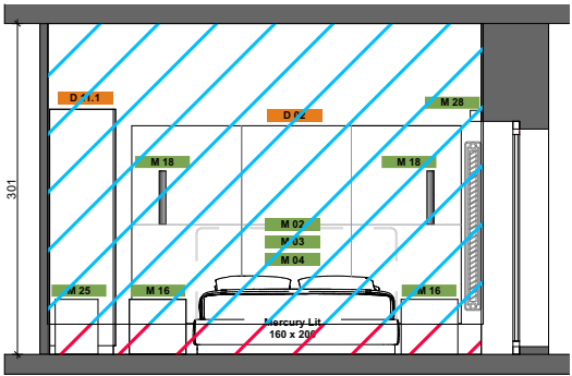
ELEVATION A-A 1: 75
