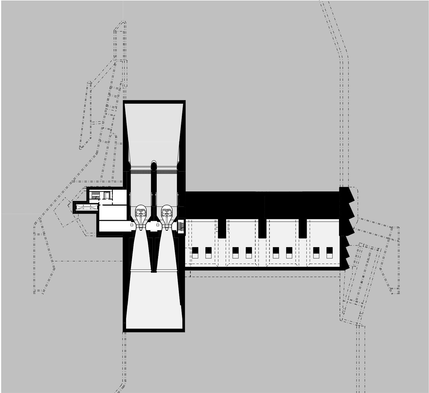
1:500 Grundriss_ +0.00
