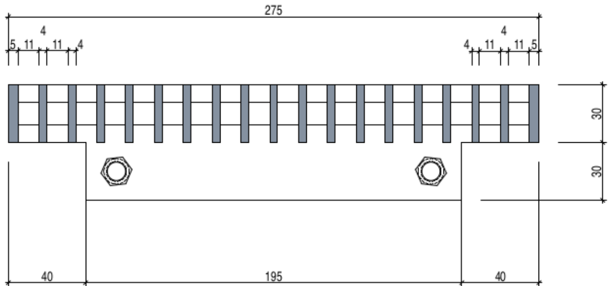
DETTALIO GRADINO 1/2
