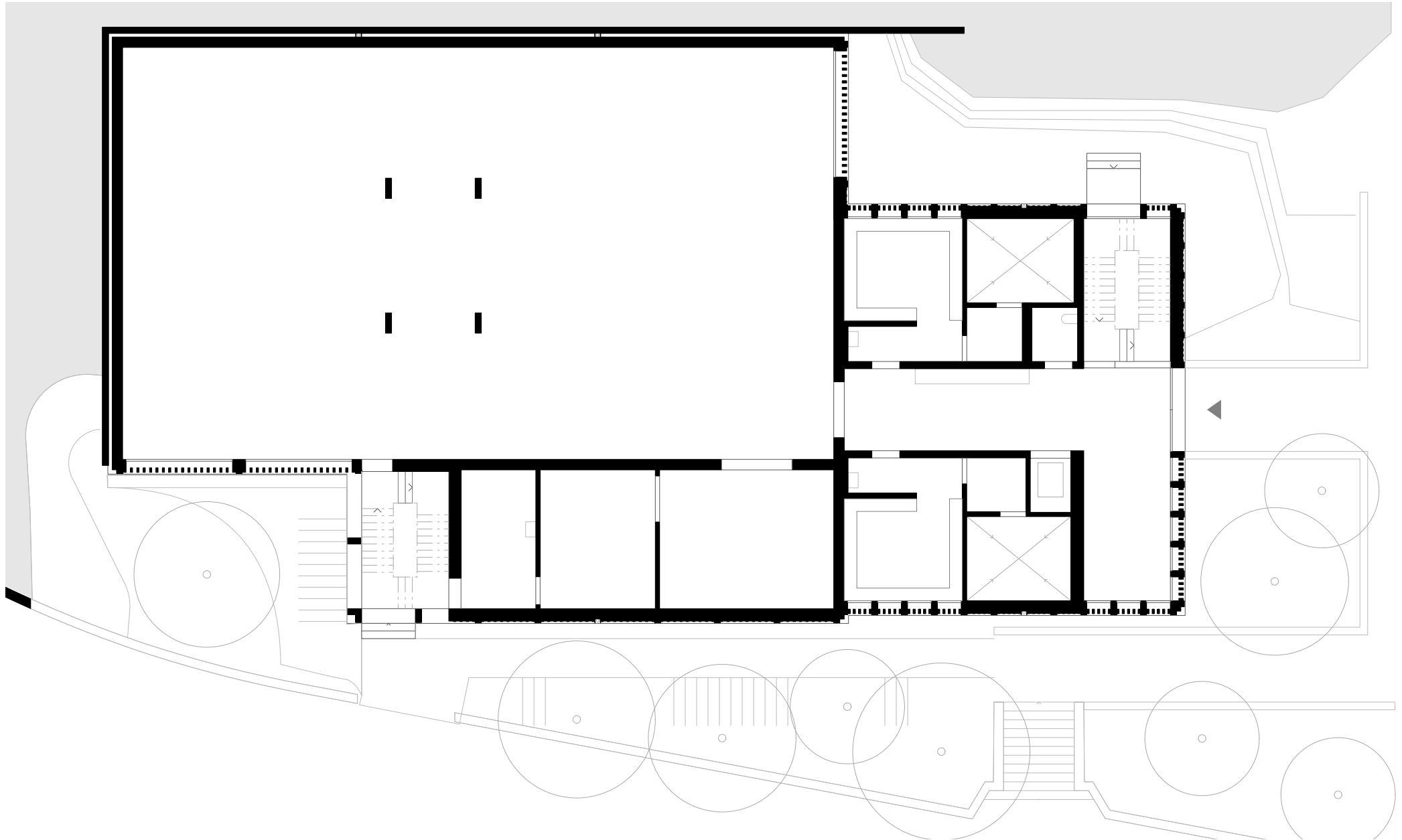
Grundriss - Erdgeschoss Ground Floor Plan
