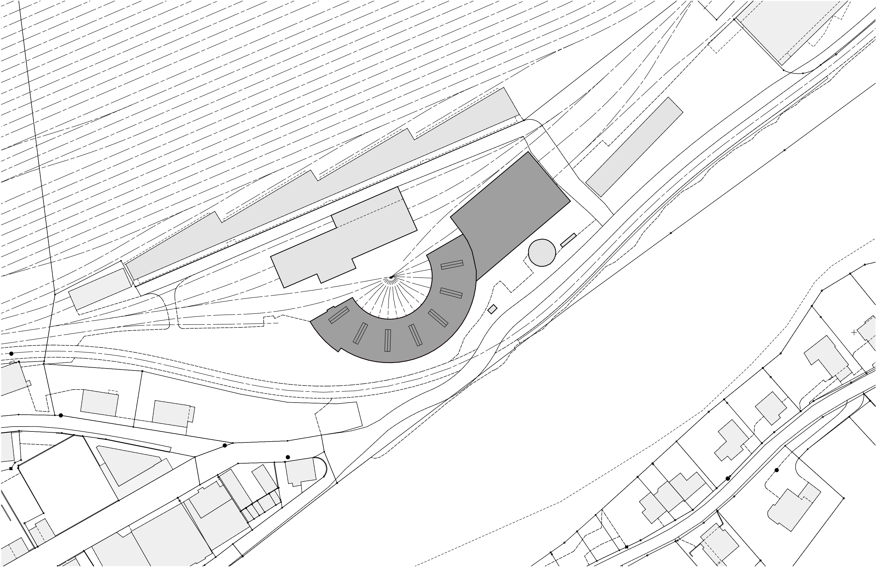
Situationsplan 1:1000
