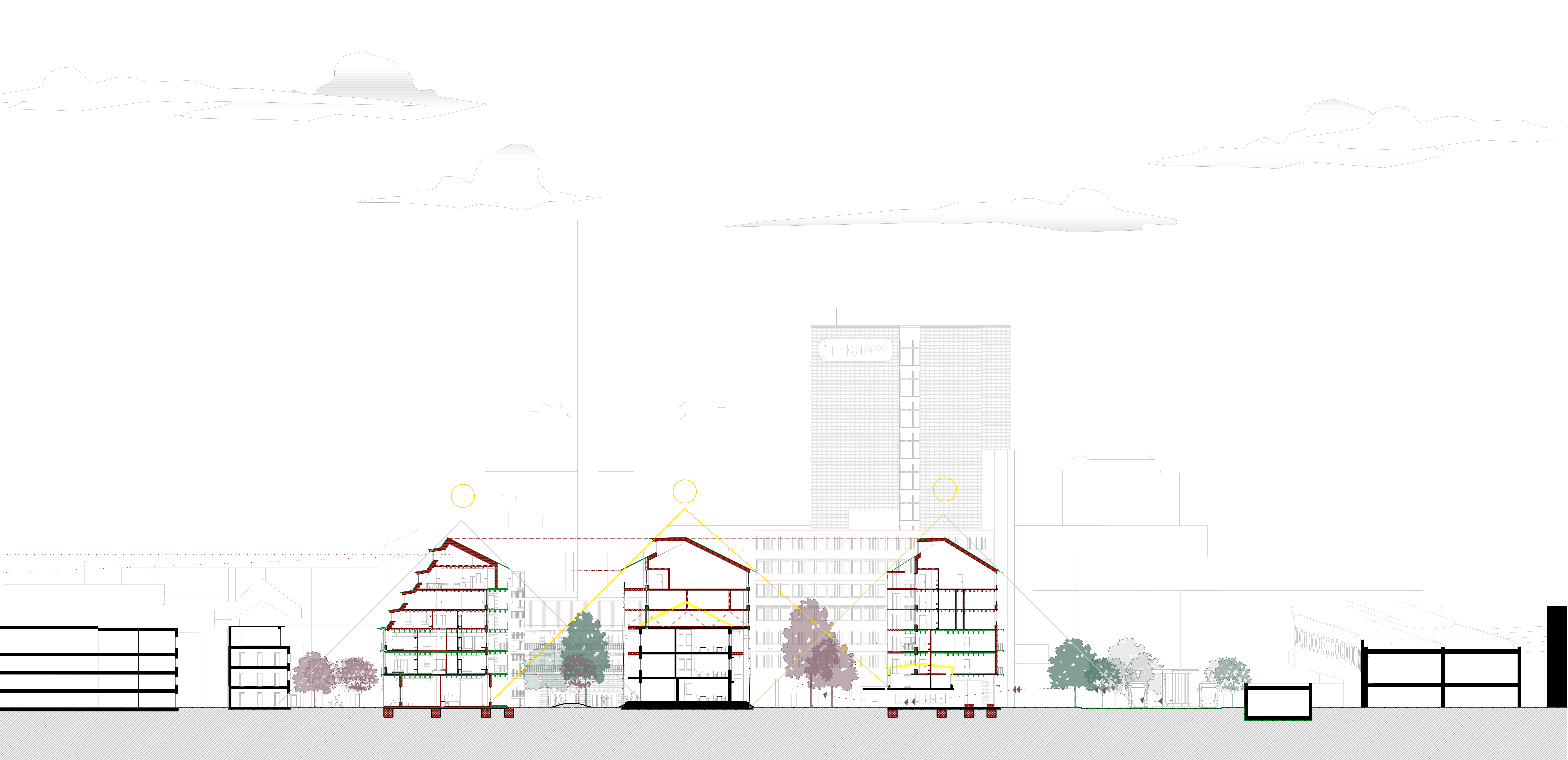
section 1_200
