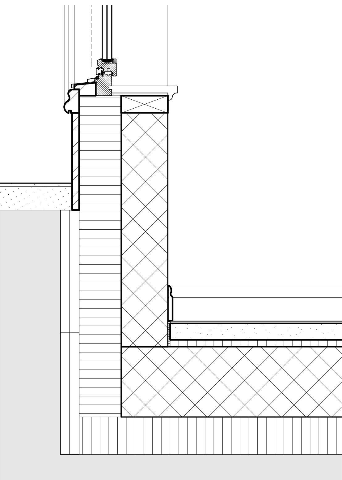
Sockeldetaill 10
