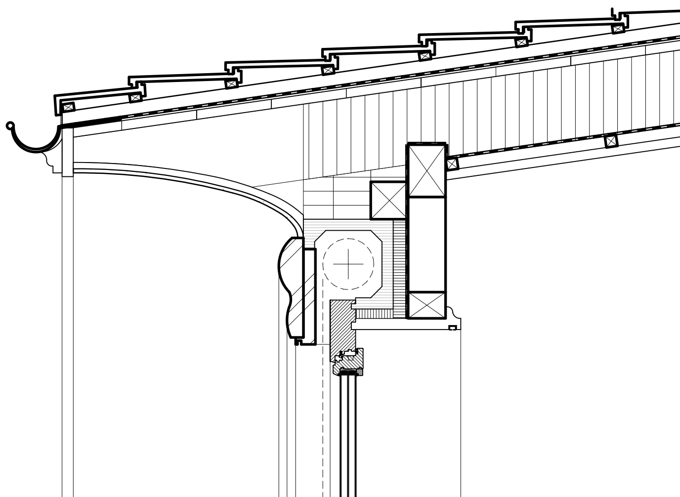
Dachranddetail 10
