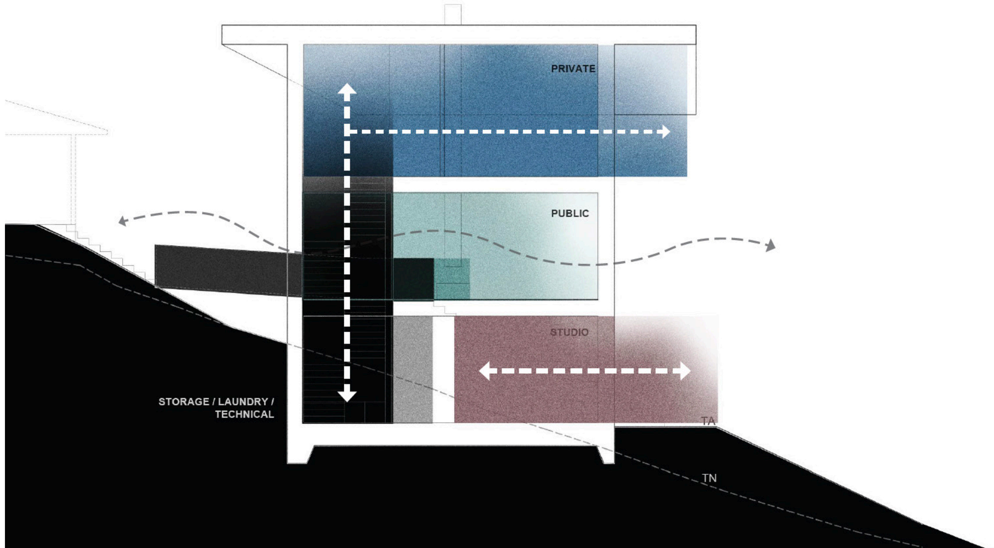
BUILDING SECTION
