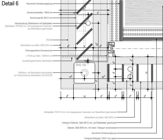
Detail 6
