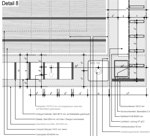
Detail 8
