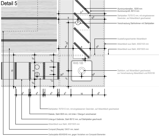
Detail 5
