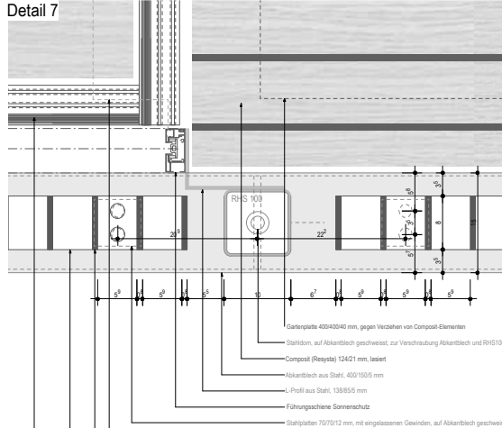
Detail 7
