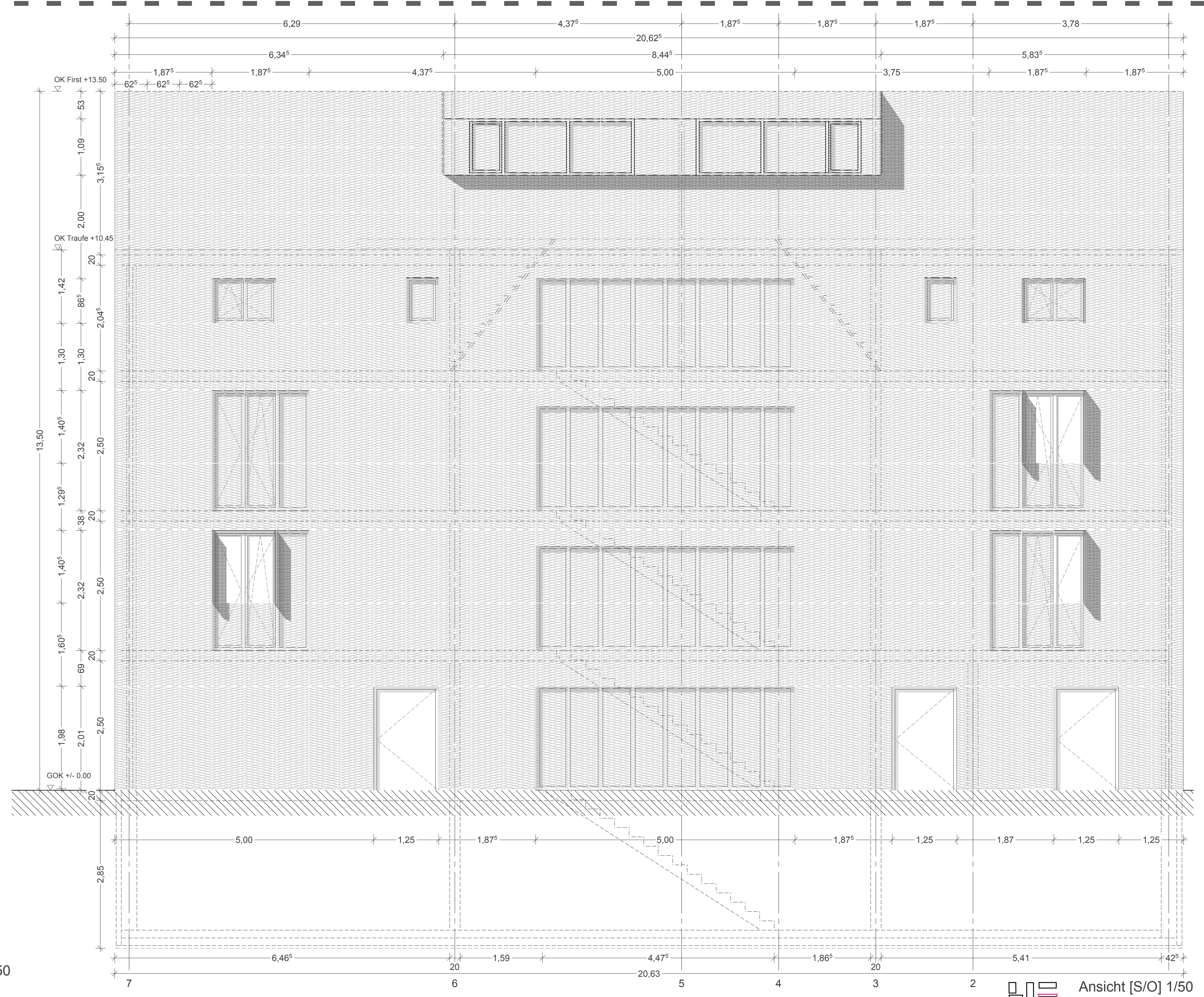
Ansicht [S/O] 1/50
