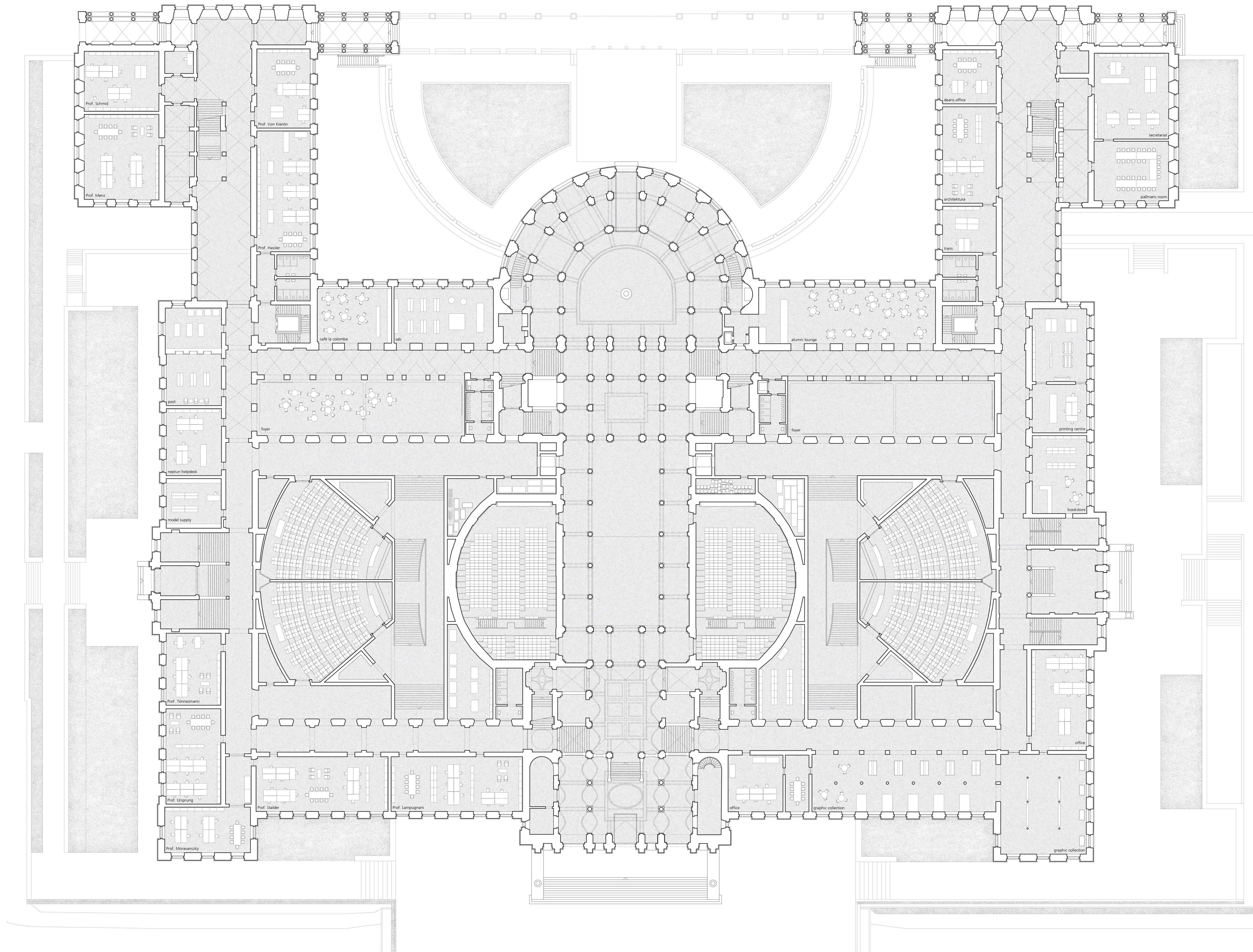
ground floor plan 1:200
