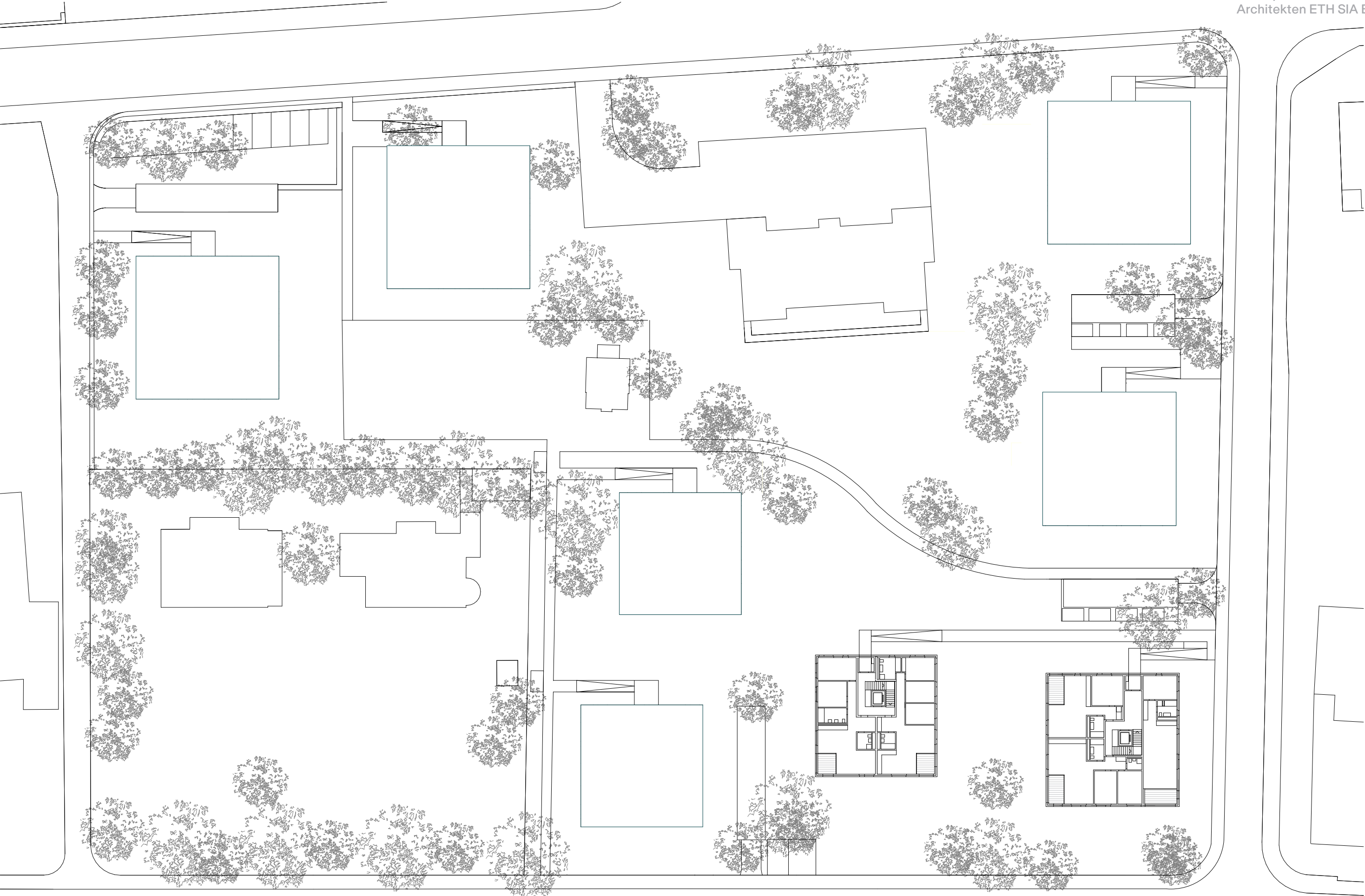
Erdgeschoss_B3_C2
