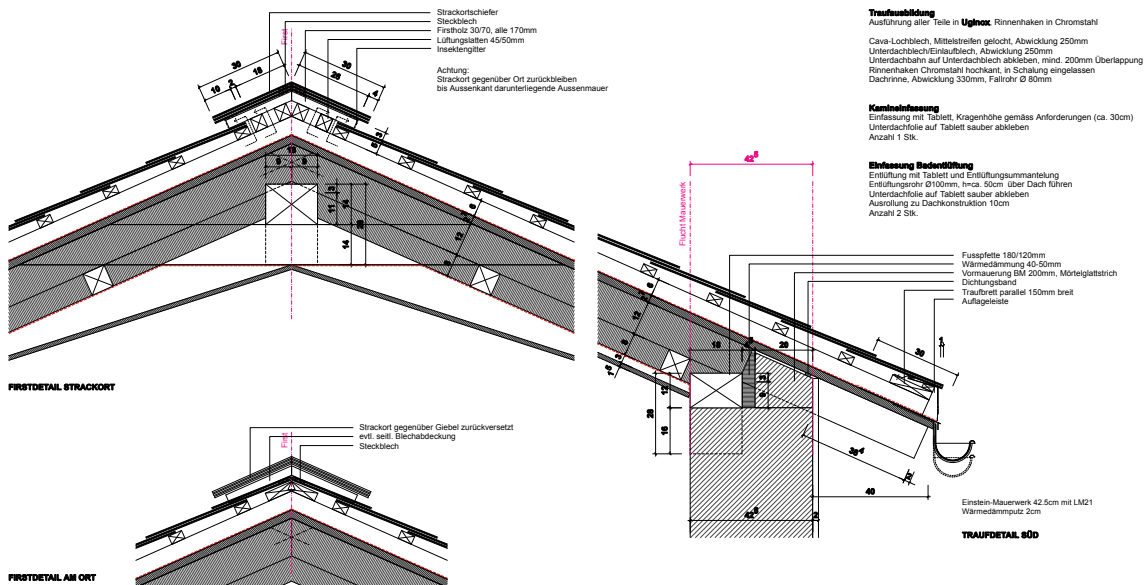
DETAILS FIRST/TRAUFE
