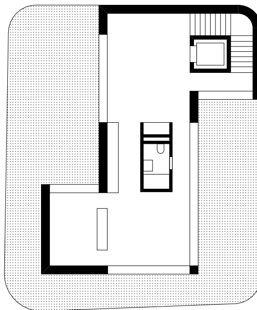
Grundriss Attika
