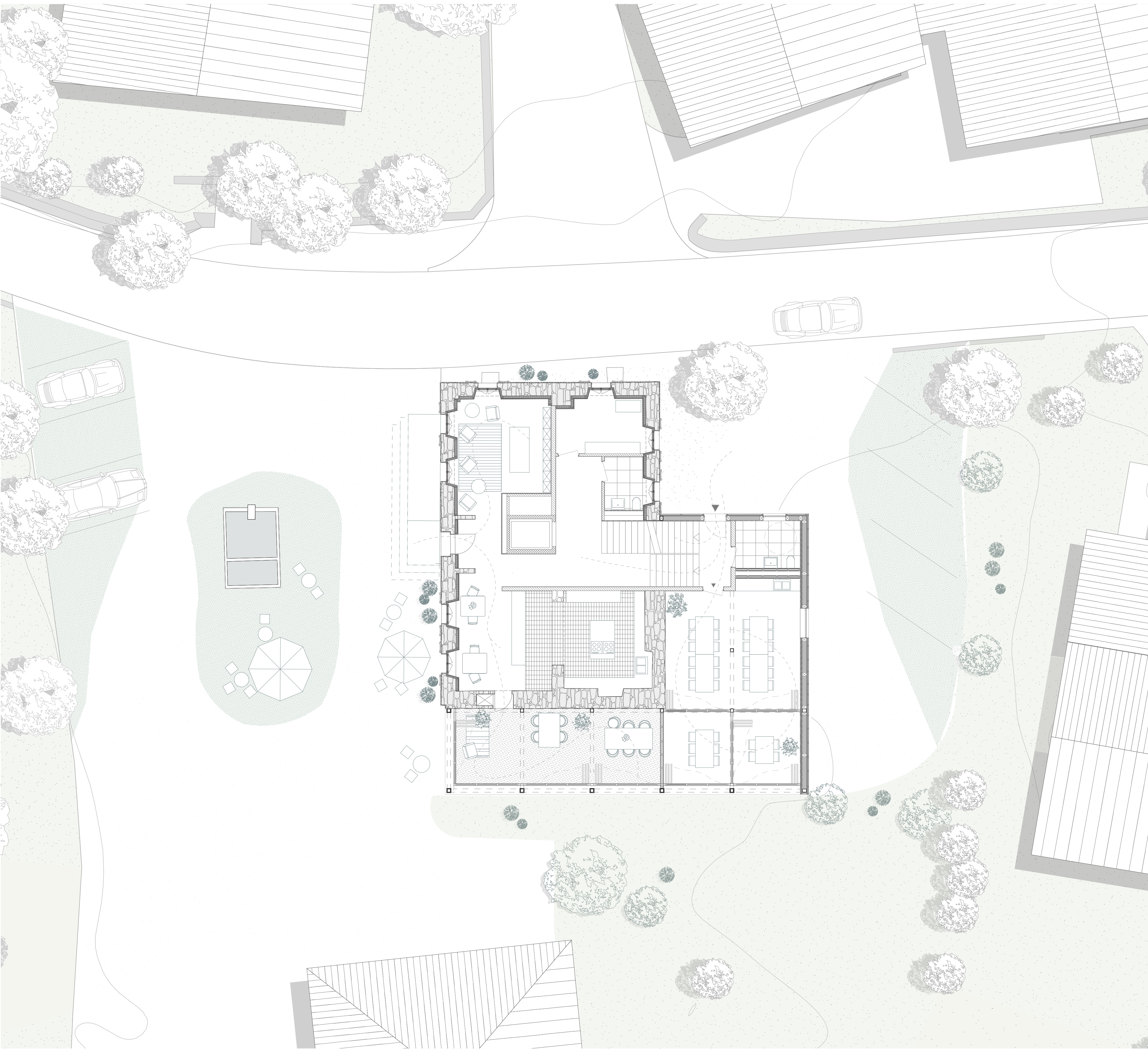
Situationsplan 1:500
