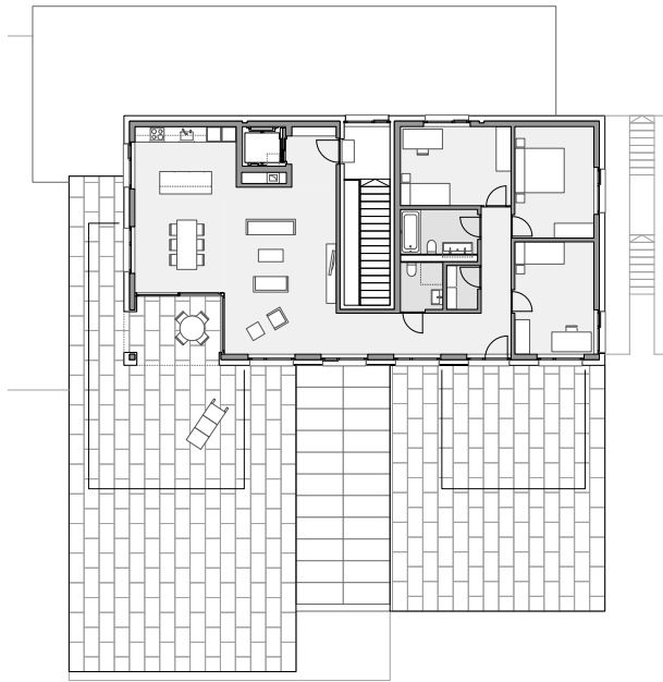
Attikageschoss
