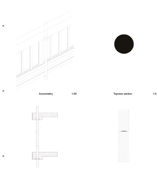
Radiator Cover Grille
