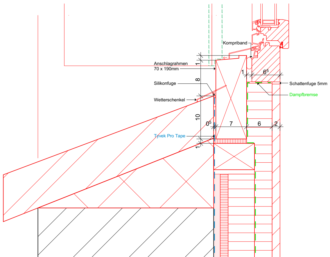
Detail Fenster EG 1:5
