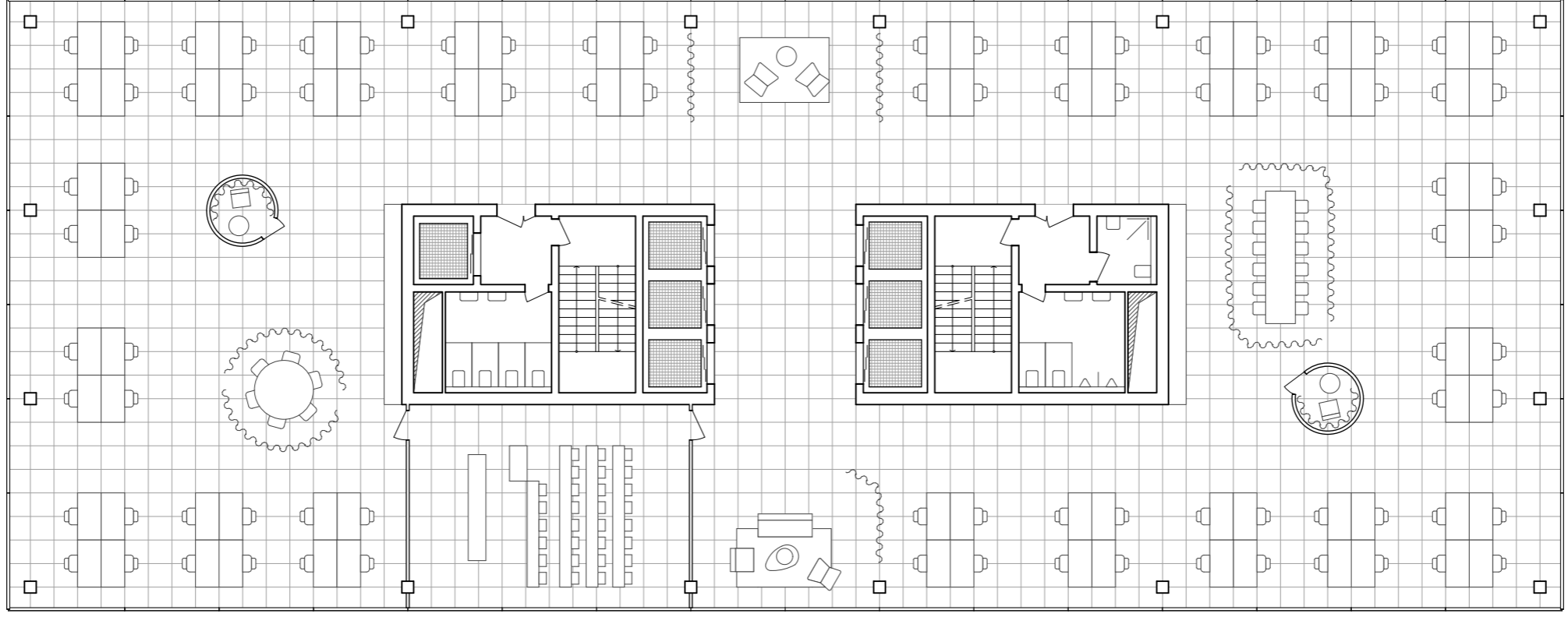
7 th to 18 th Floor office layout with meeting spaces and a seminar room
