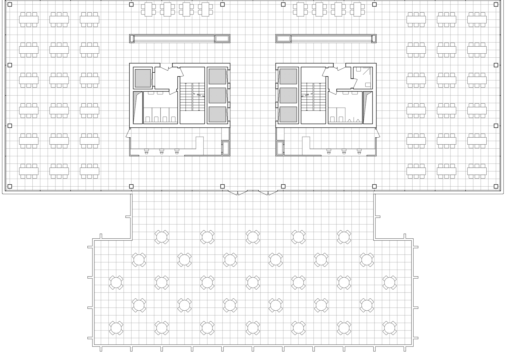
6 th Floor Cafeteria with roof terrace
