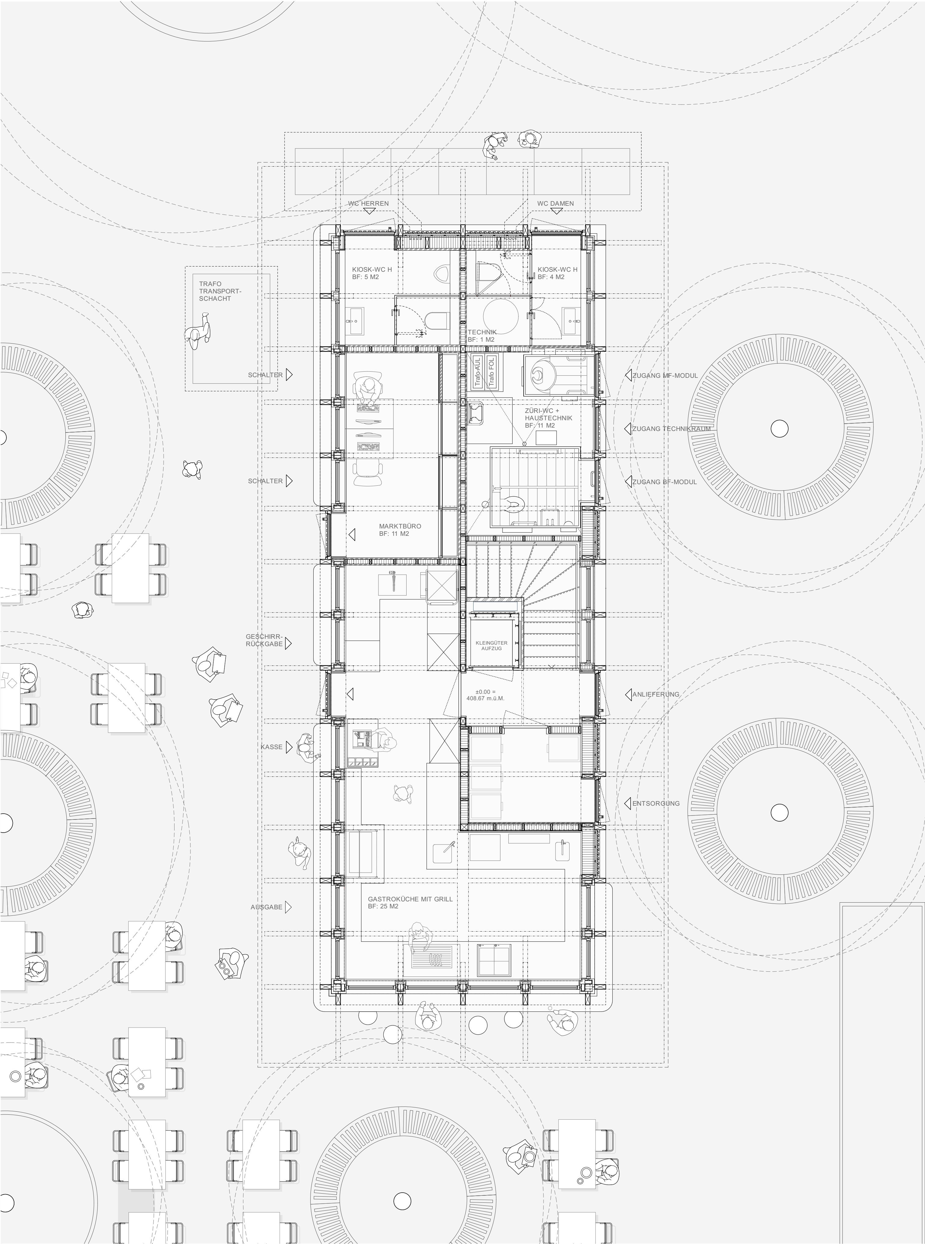
Detailgrundriss 1:50 (A2)
