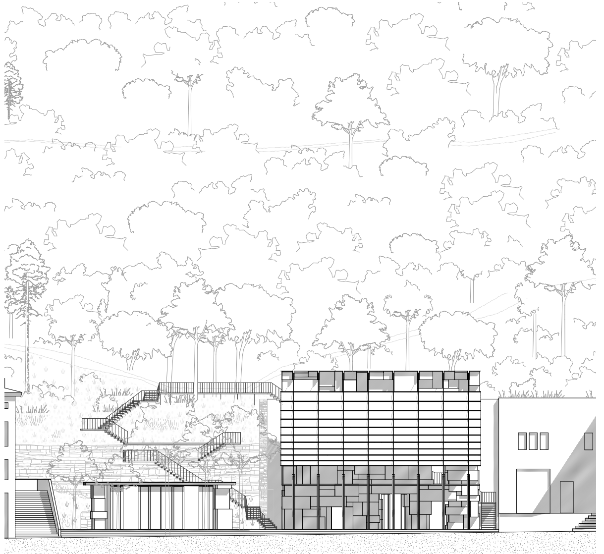
ABB. 118 Elevation
