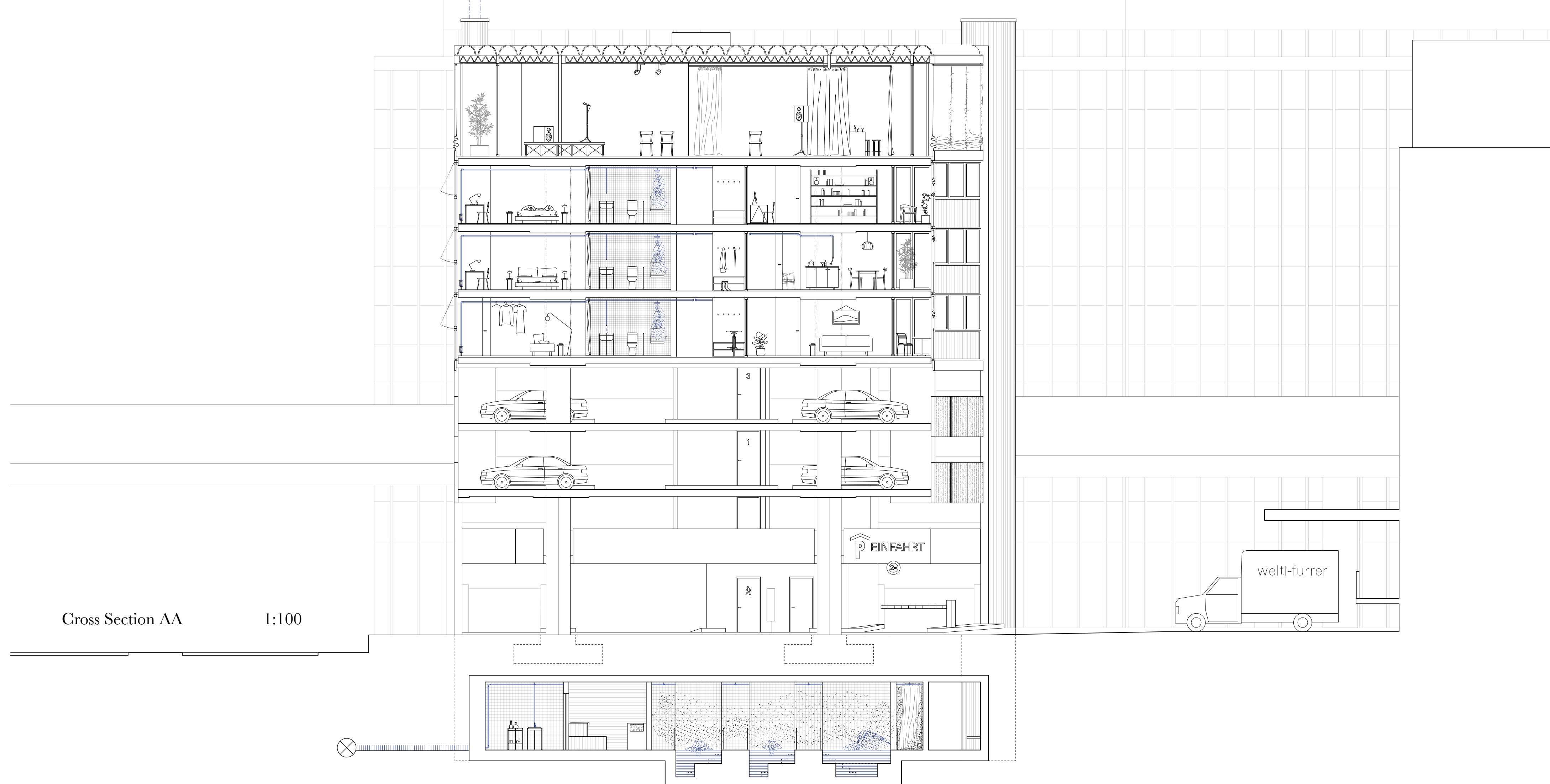
Cross Section Bathing House 1:100
