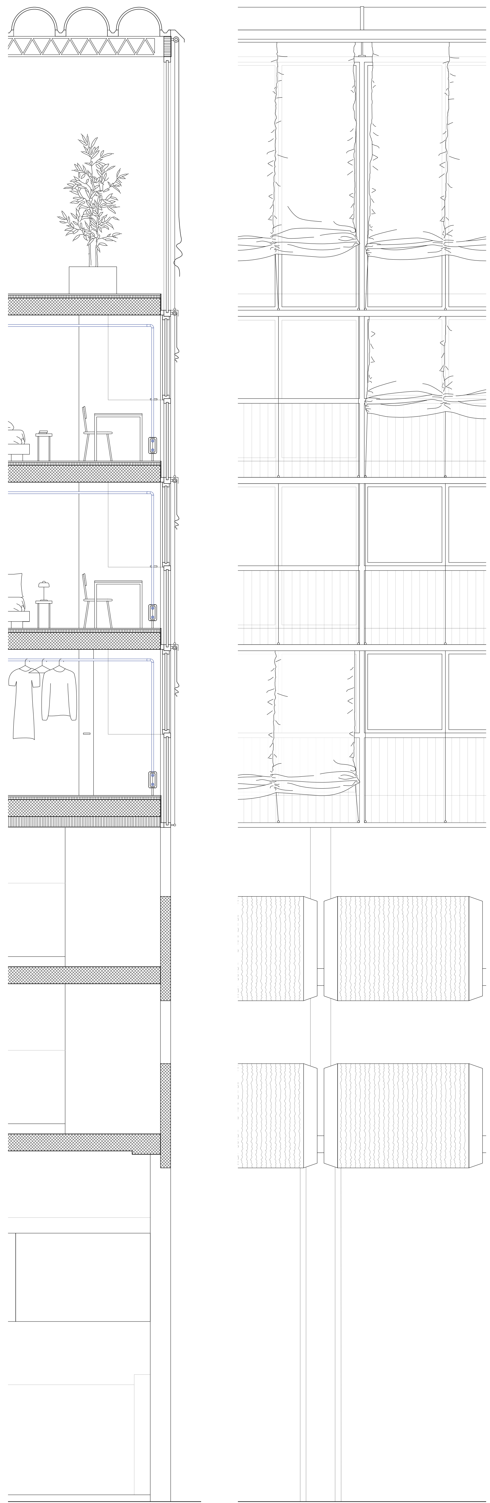
Facade Section and Elevation 1:33
