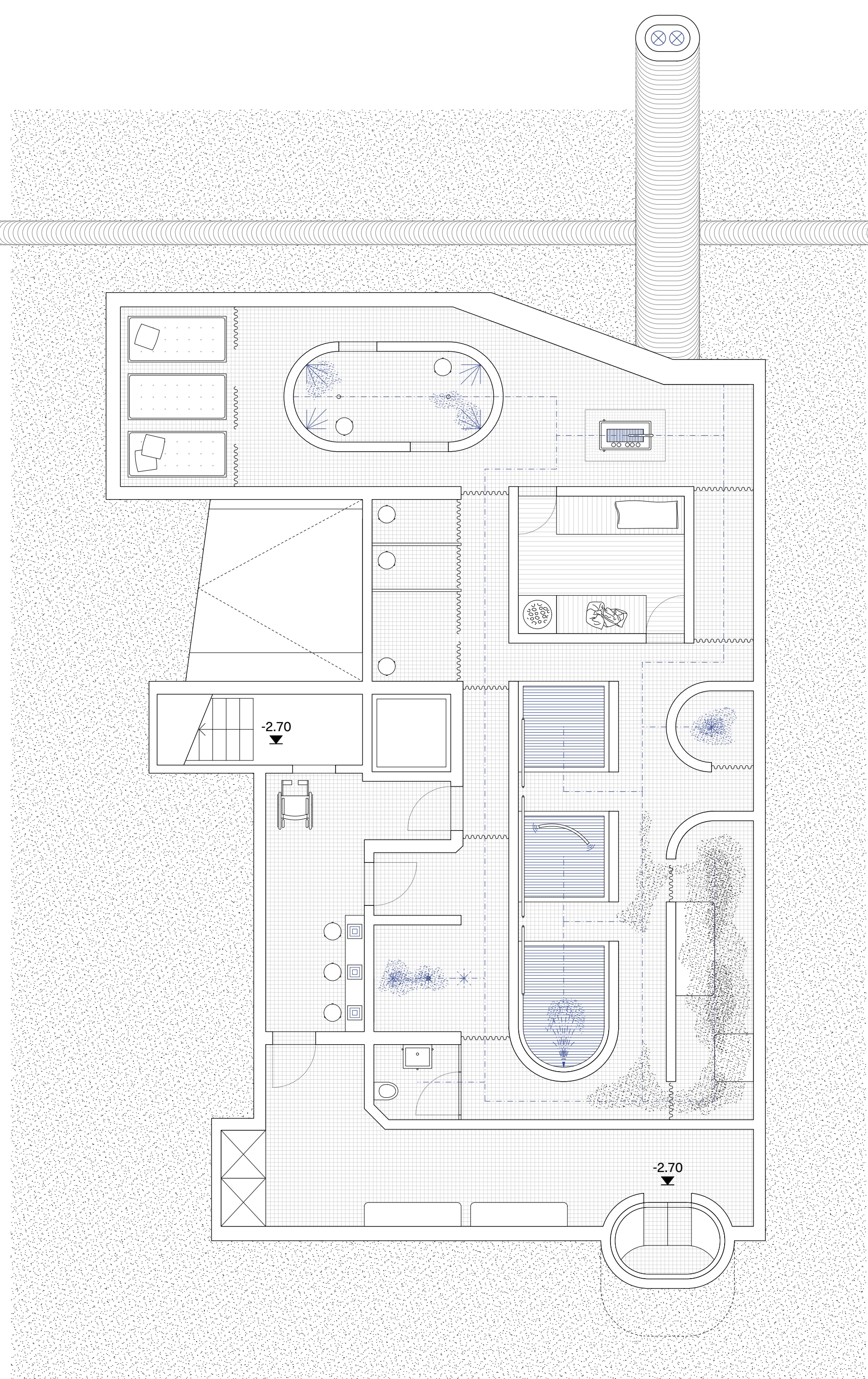
Bathing House Floor Plan 1:75
