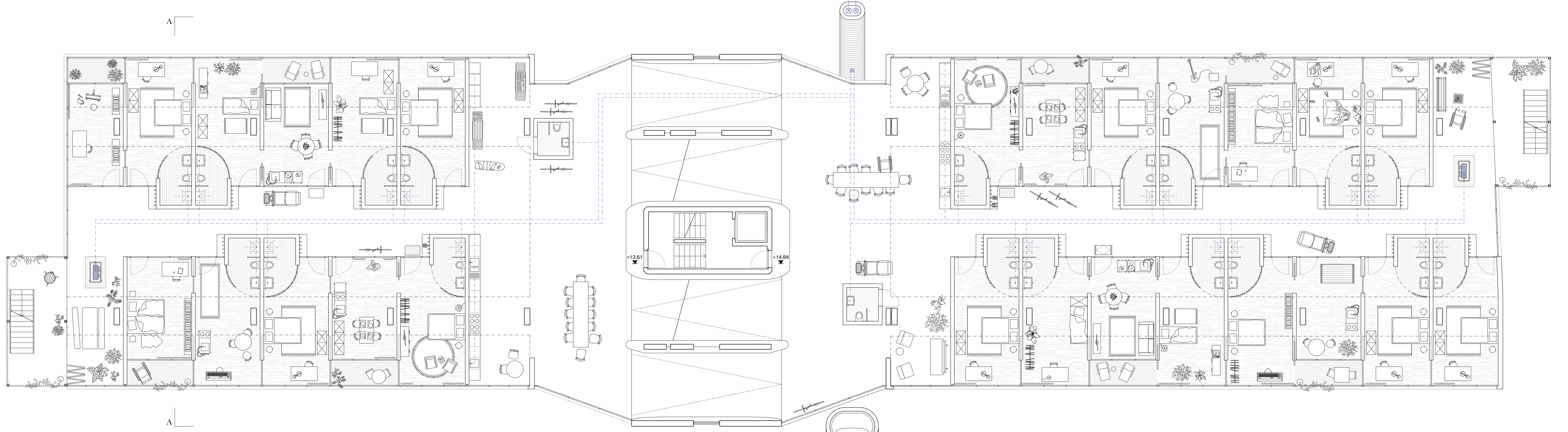
Housing/ Hotel Floor Plan (Decks 5-10) 1:100
