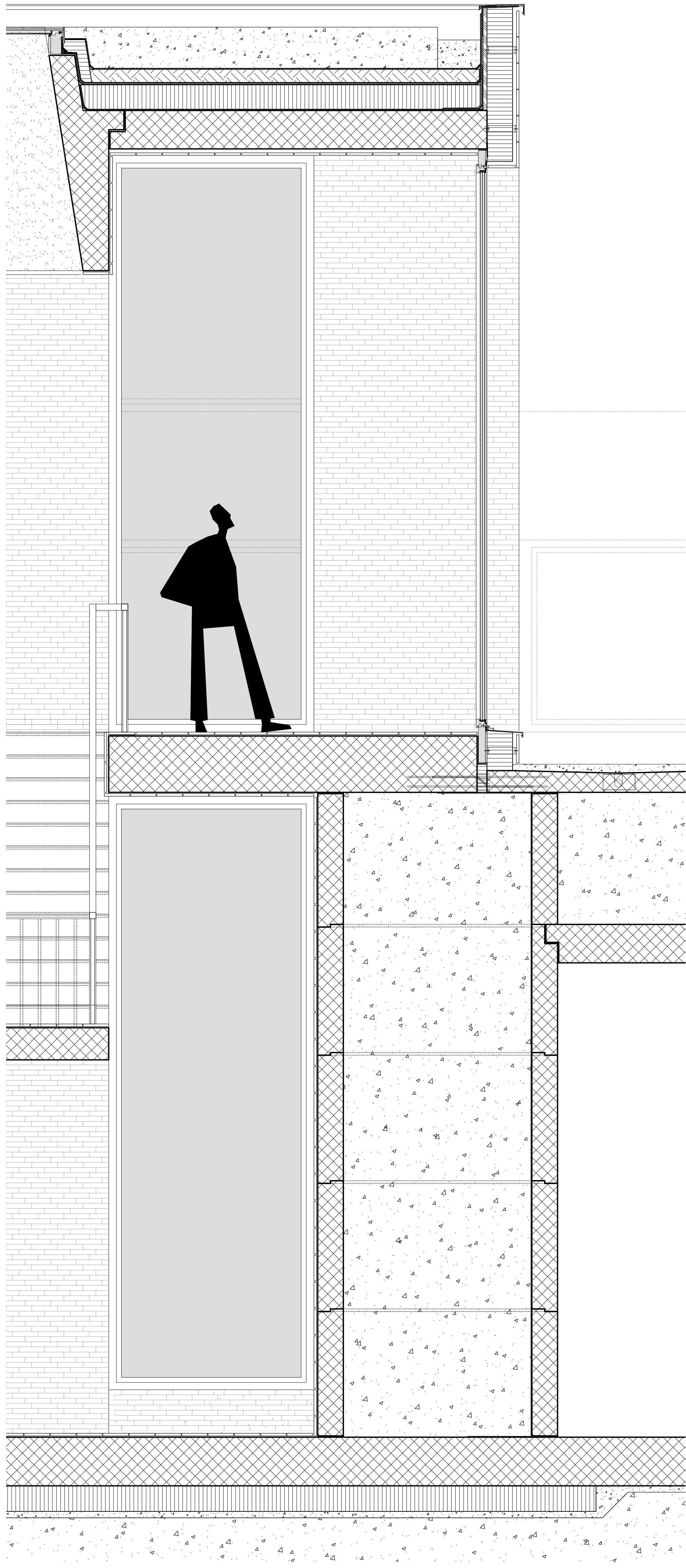
section detail 1:20
