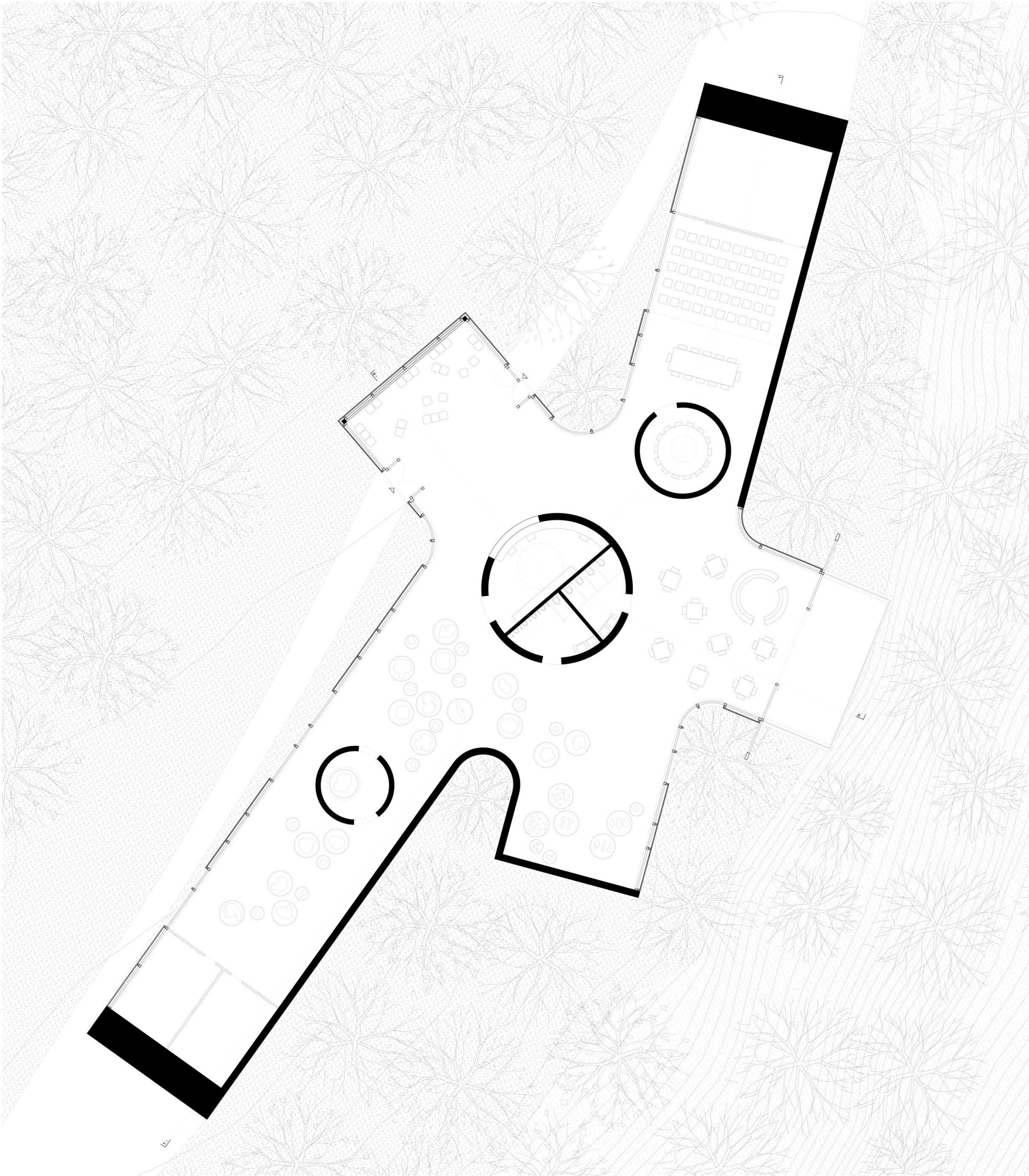
GROUND FLOOR PLAN, 1:100
