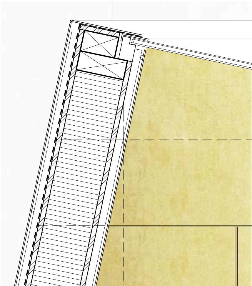
Detail roof showroom in the backyard (orig. 1:20)
