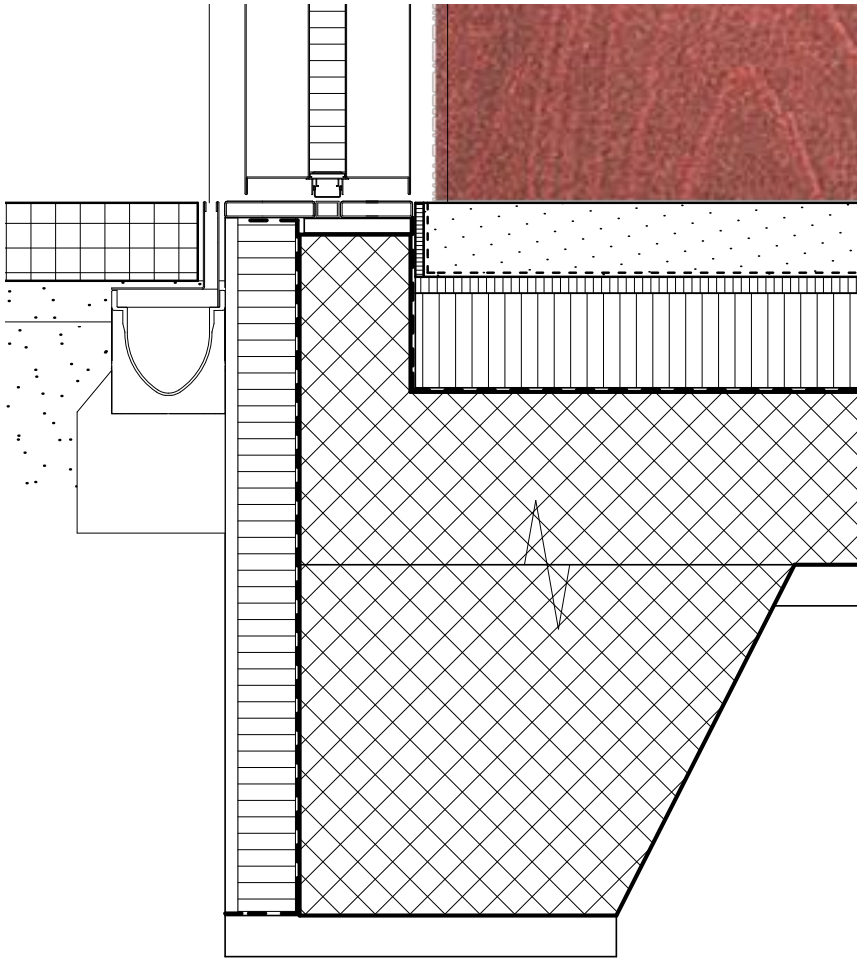
Detail base showroom on Kernstrasse (orig. 1:20)
