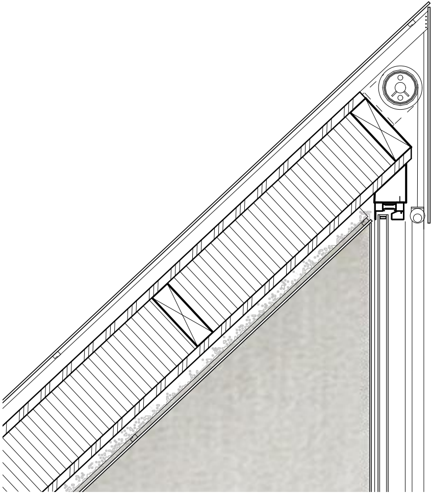
Detail roof showroom on Kernstrasse (orig. 1:20)
