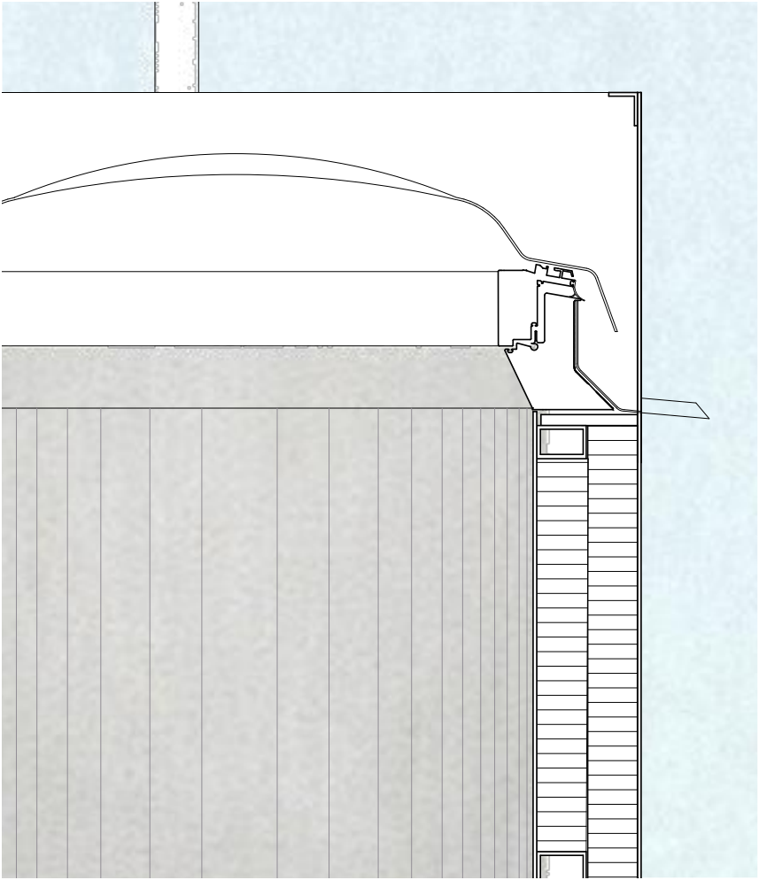
Detail round skylight innovation lab (orig. 1:20)
