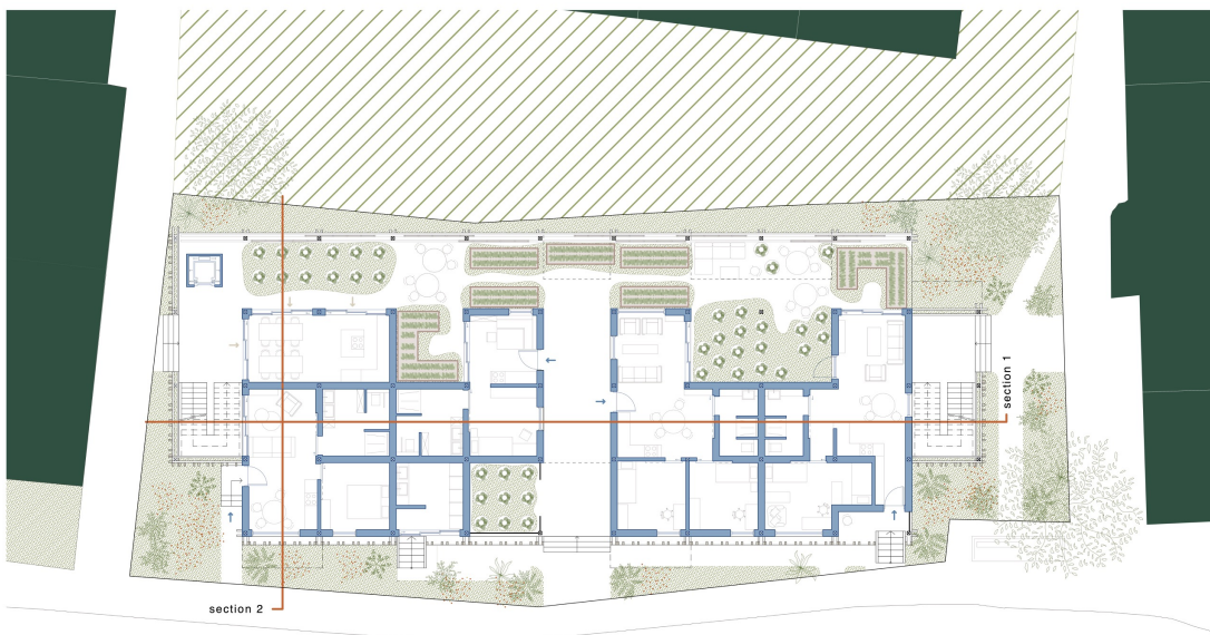
Ⓥ ground floor 1.100
