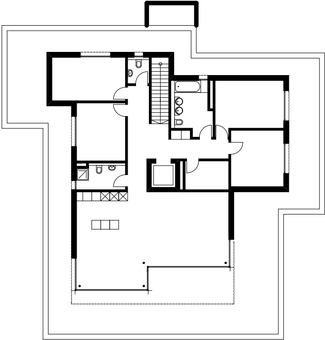
Attikageschoss
