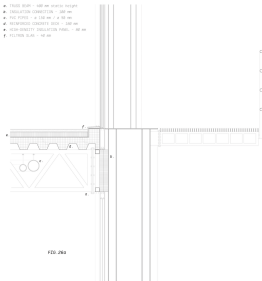
FLOOR SECTION DETAIL / HOLY TRINITY DETAIL
