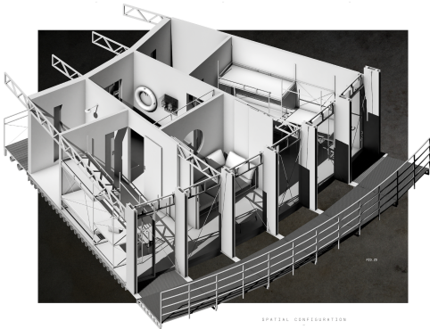
SPATIAL CONFIGURATION
