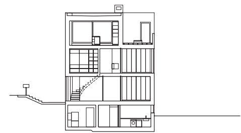
cross section
