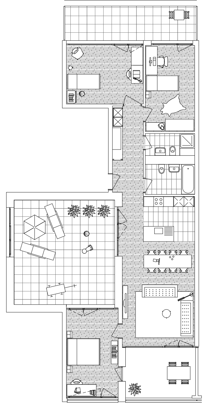
4.5 ZIMMER - ATTIKA
