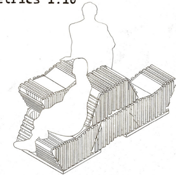
Isometrics 1:10
