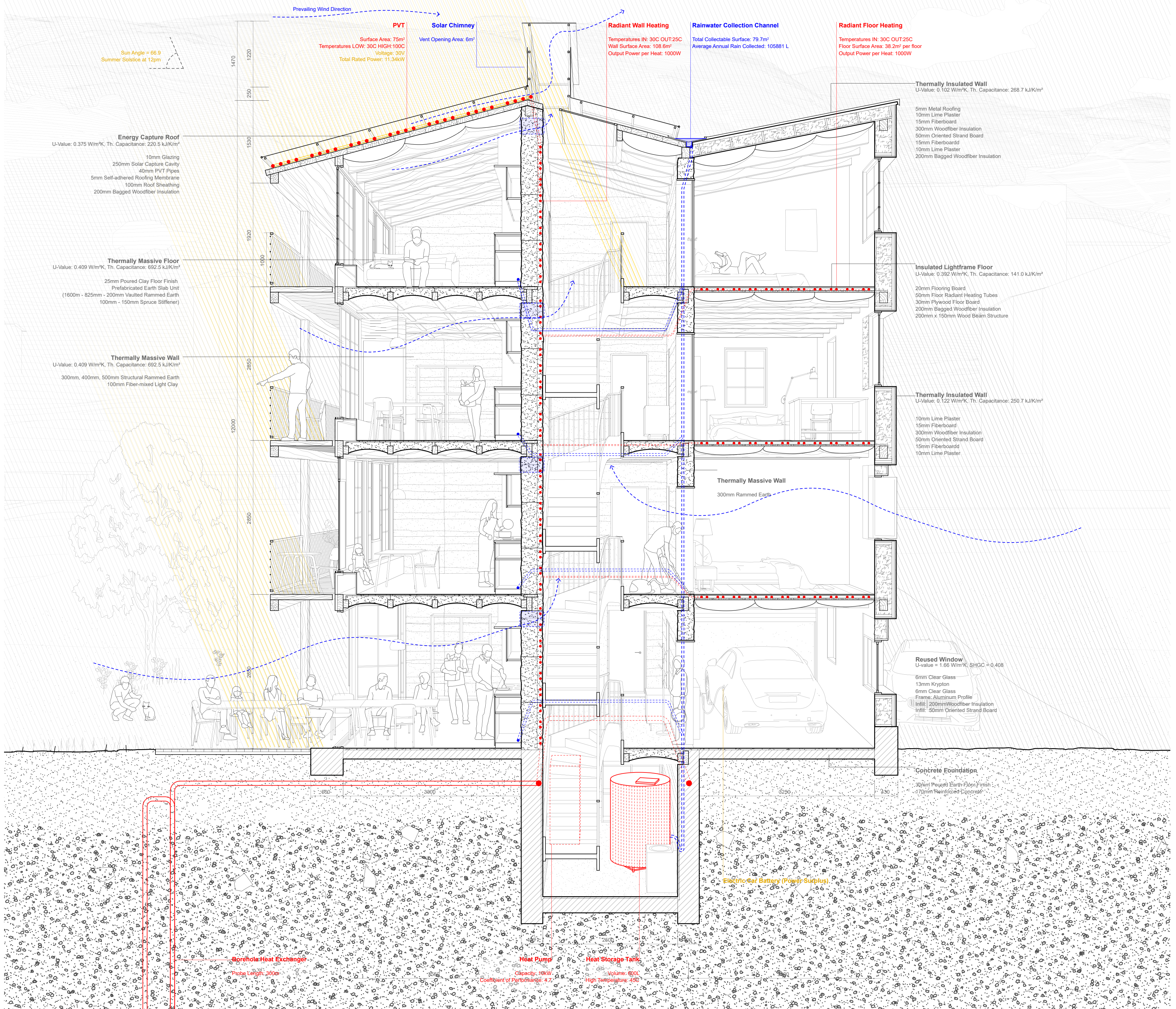
SECTION PERSPECTIVE A
