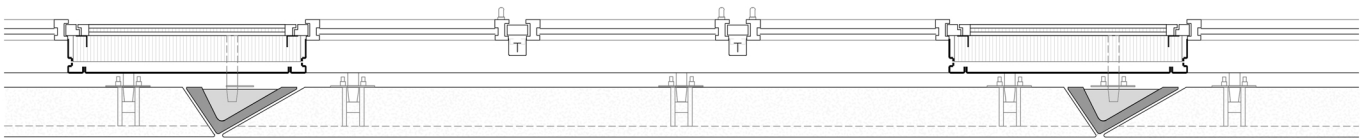
Facade concept 1:33
