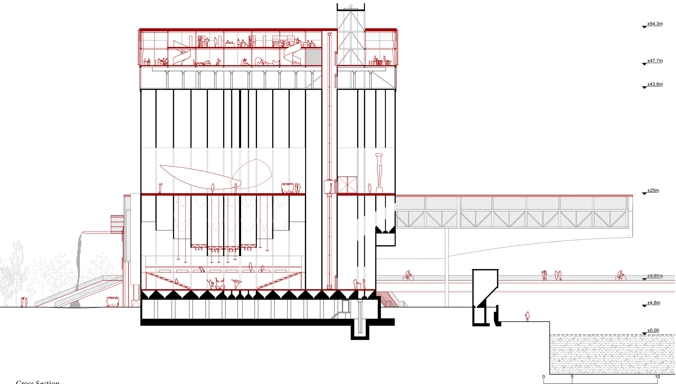
Cross Section
