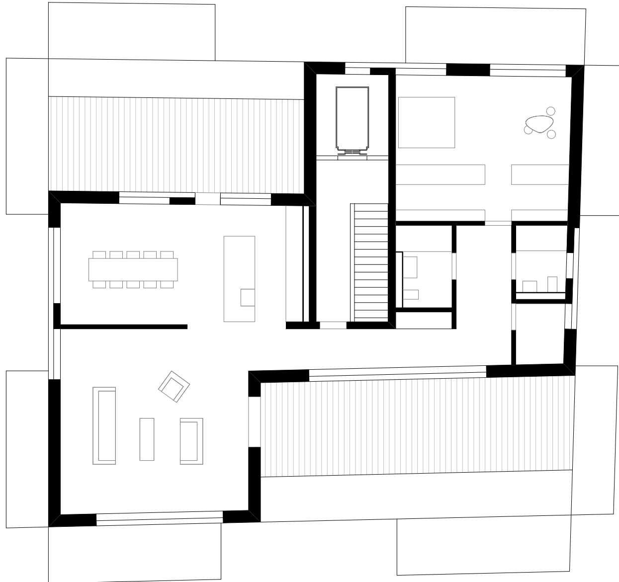
Attikageschoss
