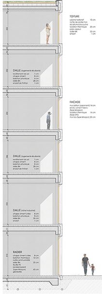
Coupe constructive - 1/50
