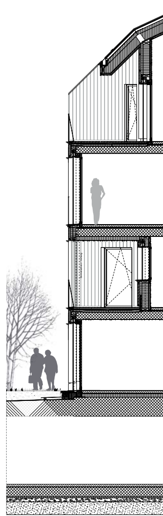
Typical section, M 1:50
