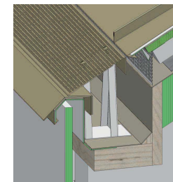
4 Roof eave gutter
