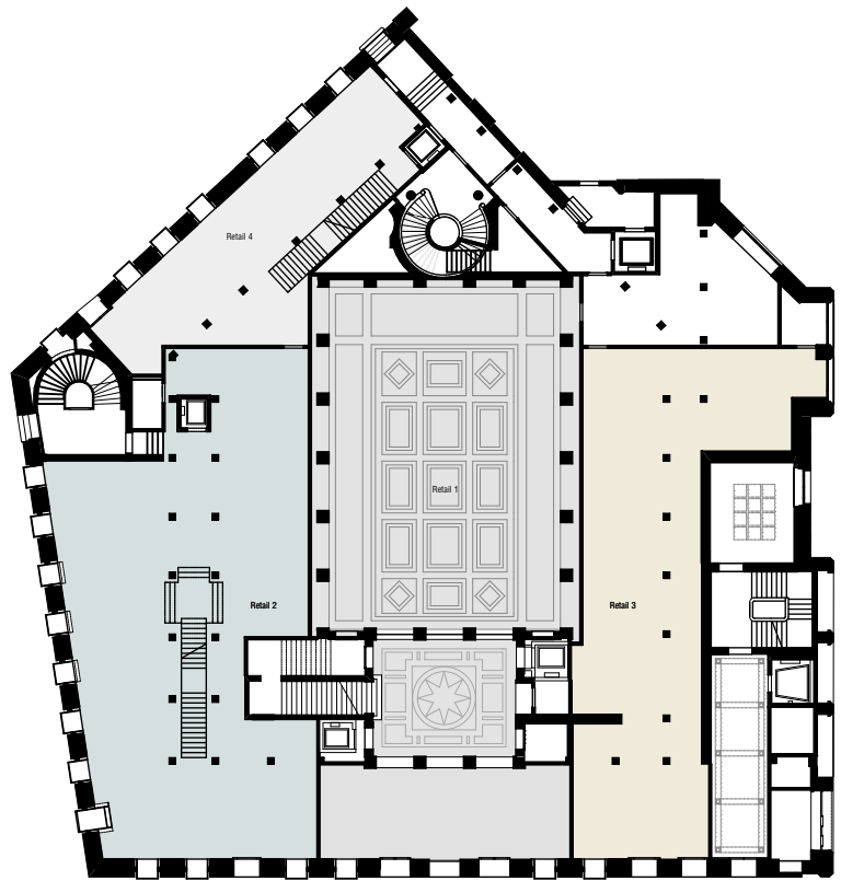
Erdgeschoss M1:500
