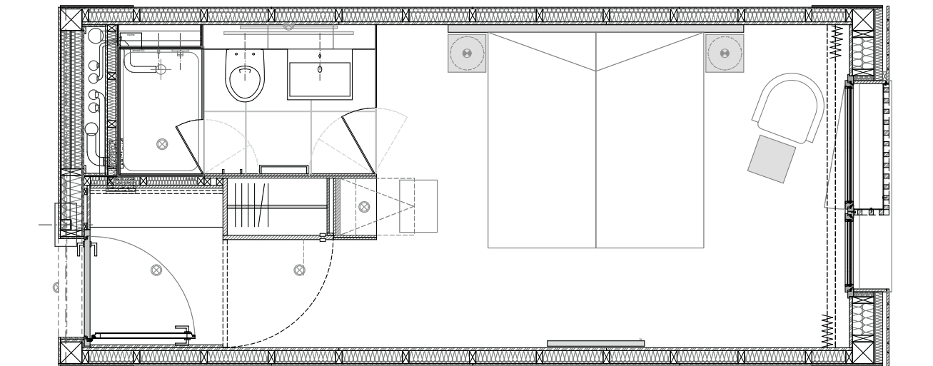
detail grundriss
