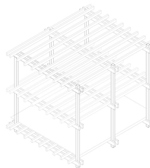
Beams and columns connection
