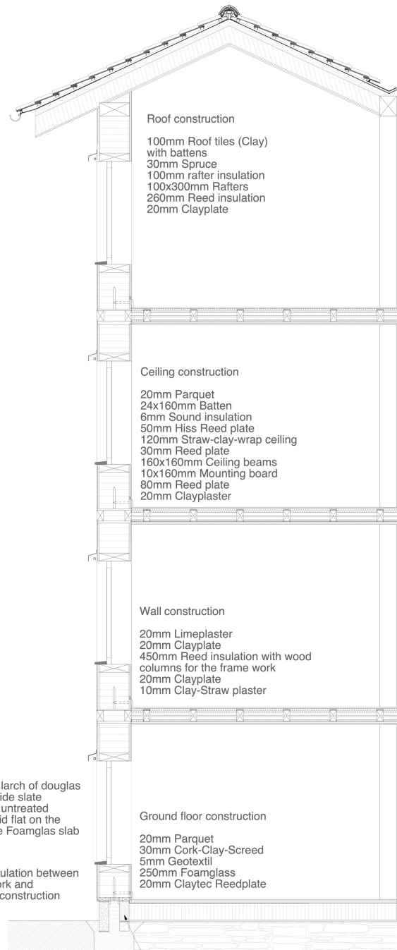
Construction Section 1:20
