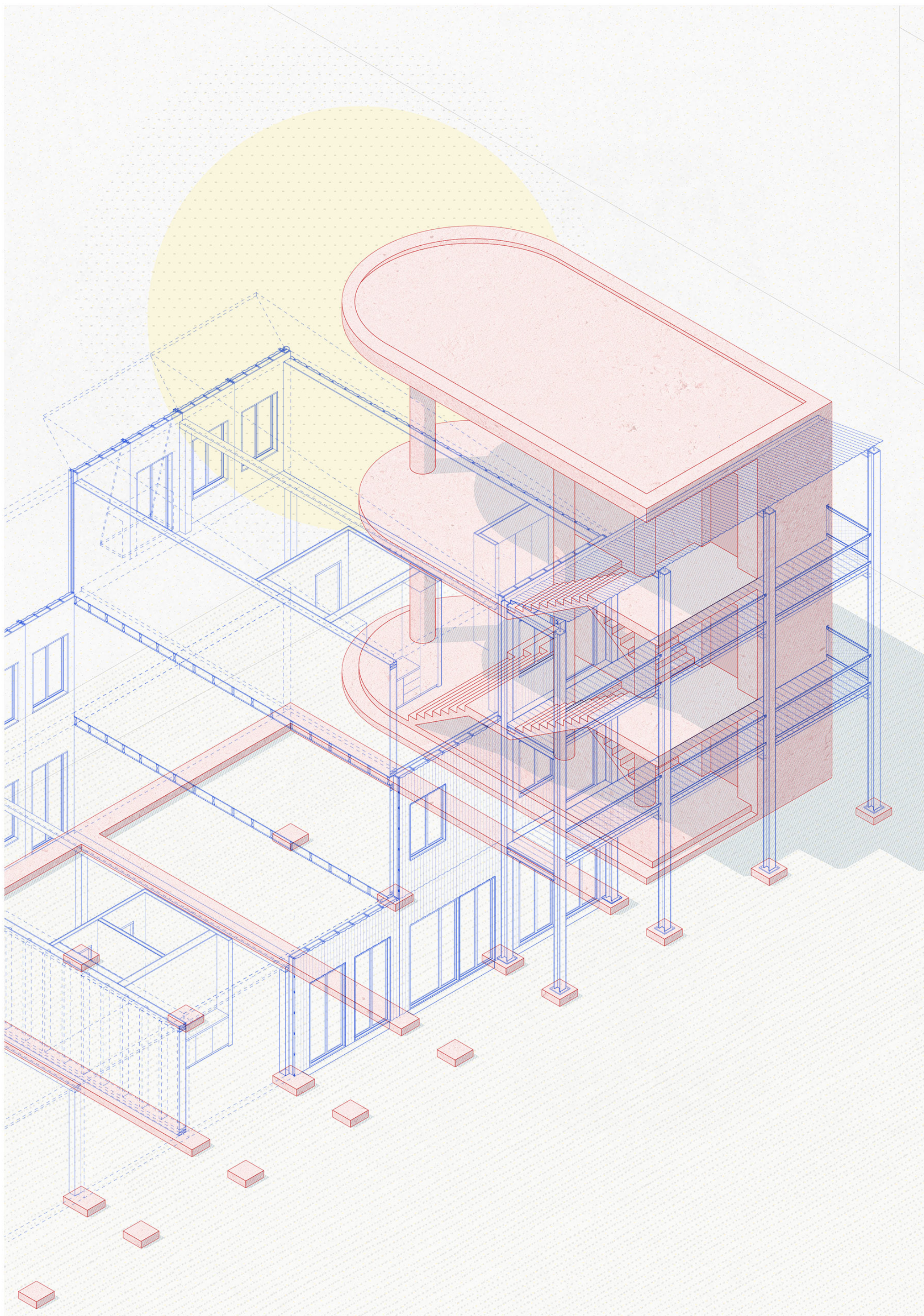
FROM MONOCULTURE TO A BUILDING ROTATION SYSTEM axonometry of the remaining element «pavillon» - overlay construction
