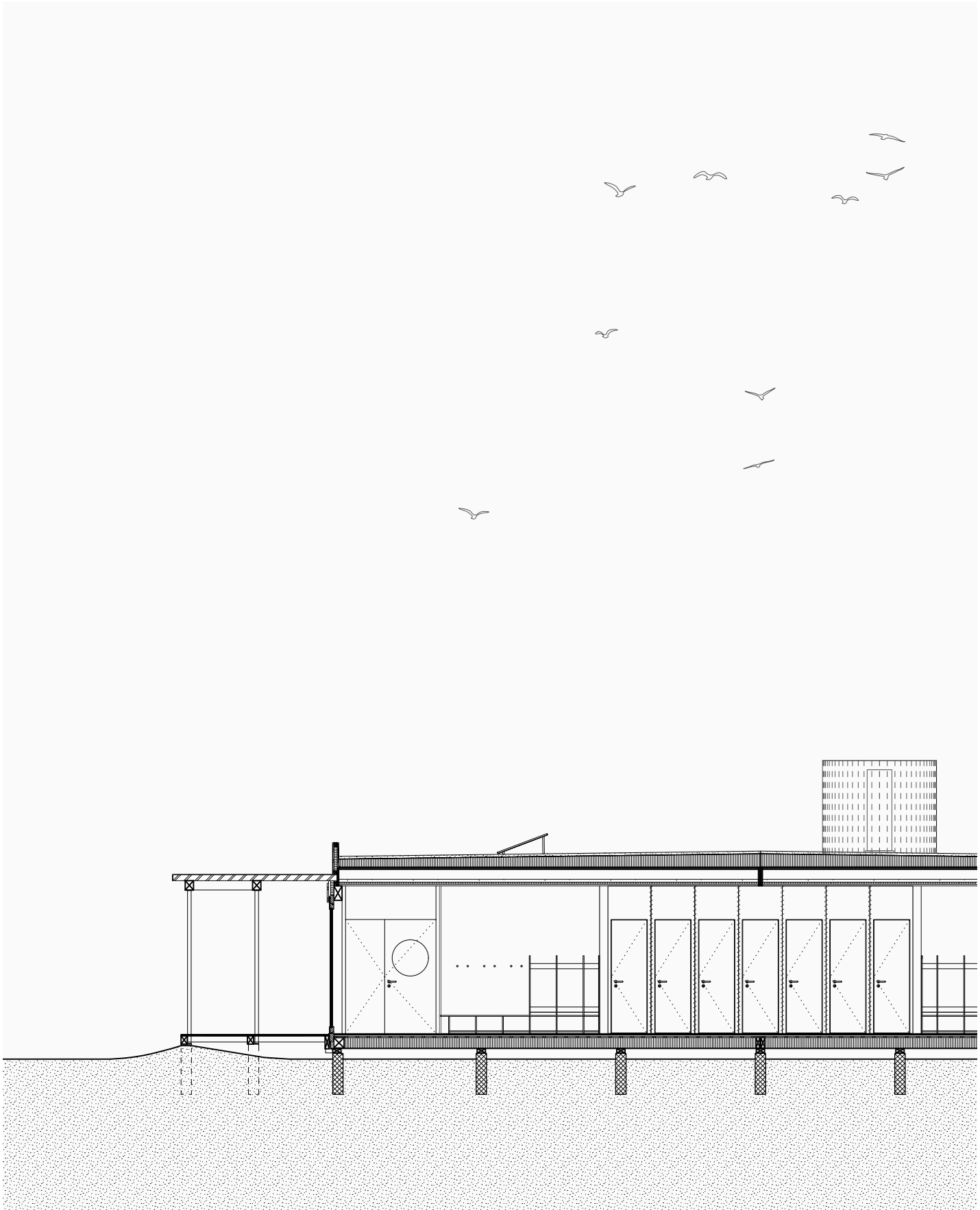
section
