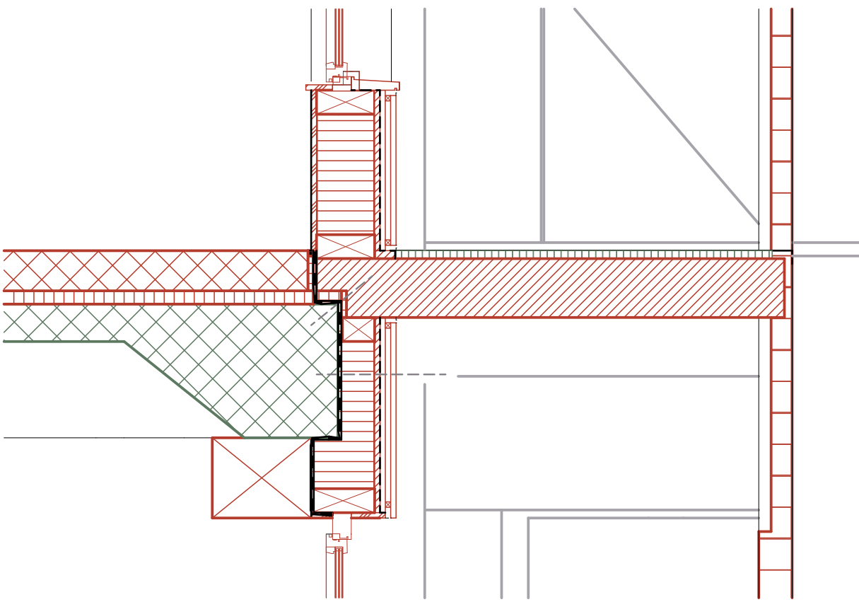
Detail arcade
