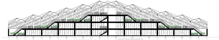
Section cut B 1:200
