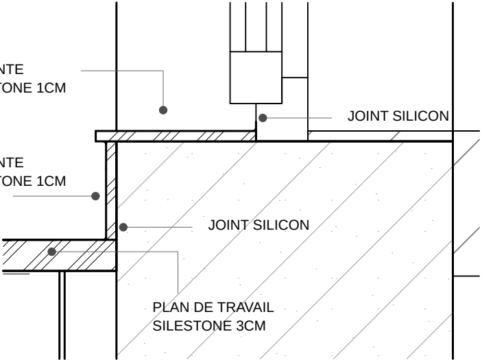
DETAIL PRINCIPE TABLETTE
