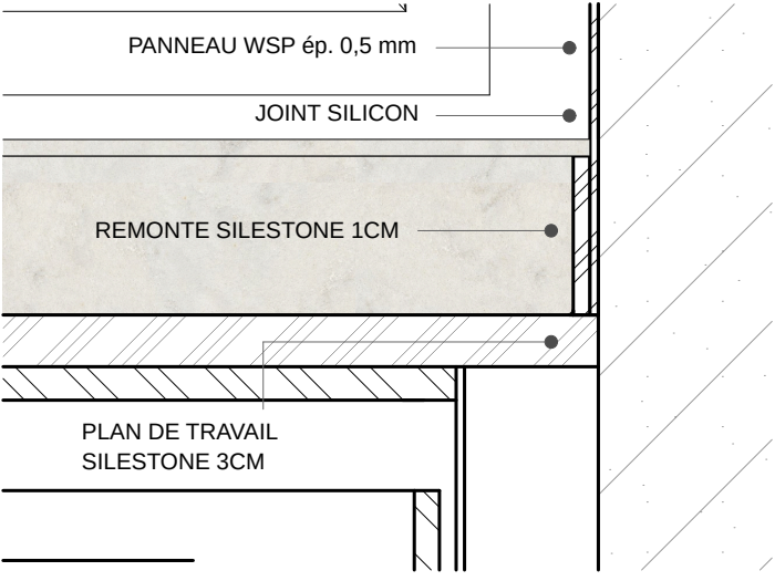
DETAIL PRINCIPE PANNEAU WSP
